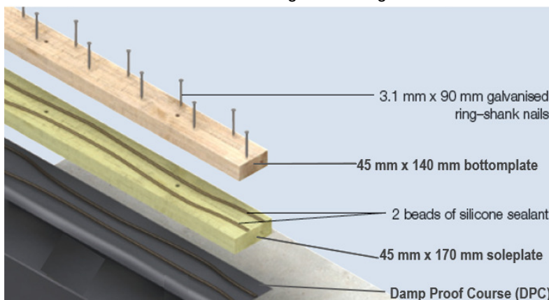
Figure 4b bottom-plate to soleplate to foundation
